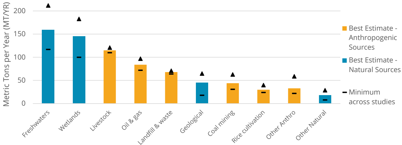
Estimated Sources of Methane, 2000-2006
